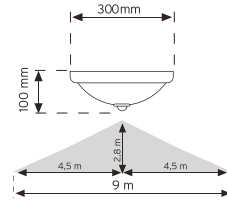
AK-04 Hareketli Sensörlü LED Ampul Kitli Tavan Armatürü Sensored Lighting With LED Lamp
